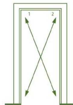
FIGURE 2 Is the door frame square? Check by measuring diagonally as illustrated. If the frame is out of square, you may require a slightly larger door and trim it to size. A trimming allowance of up to 3mm is allowed on all doors.
