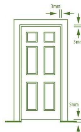
FIGURE 3 Important: Approximately 3mm clearance is required at the top and sides of the door and 5mm at the bottom (above the floor covering).
