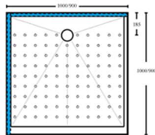
FPSSL1000-2W Left Hand Corner FPSSL900-2W Left Hand Corner
