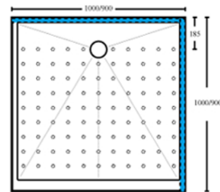
FPSSL1000-2W Right Hand Corner FPSSL900-2W Right Hand Corner
